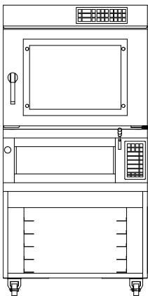
MIWE bakecombi consisting of: econo 10.1826 / condo 1.0608 underframe / rollers
